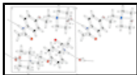
Fig. 2. Crystal packing of the title compound with intermolecular N-H \cdots O , O-H \cdots O and O-H \cdots N hydrogen bonds shown as dashed lines.
