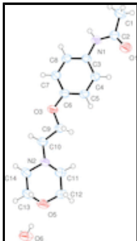
Fig. 1. The molecular structure of the title compound. Displacement ellipsoids are drawn at the 50% probability level.
