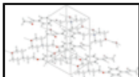
Fig. 3. Crystal Packing of the title compound viewed along the b axis.
